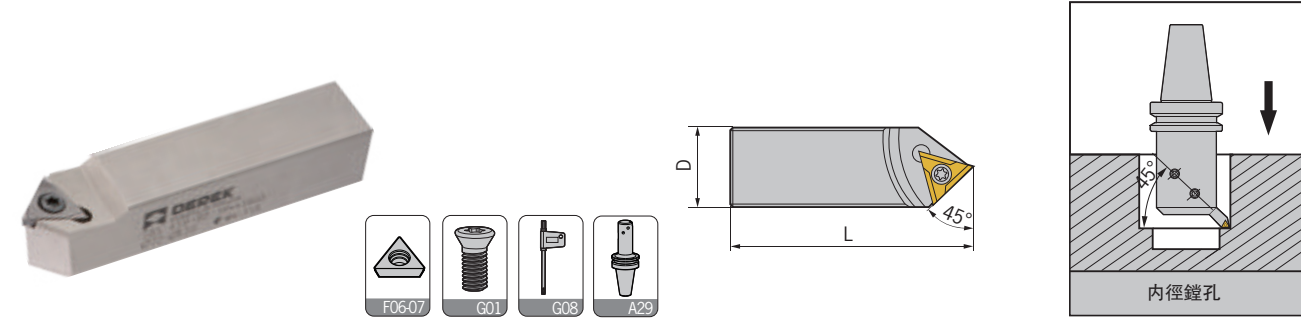
T45度刀杆適用於BSA刀柄 For BSA Boring Holder
