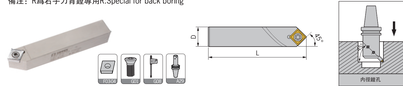
C45度刀杆適用於BSA刀柄 For BSA Boring Holder
