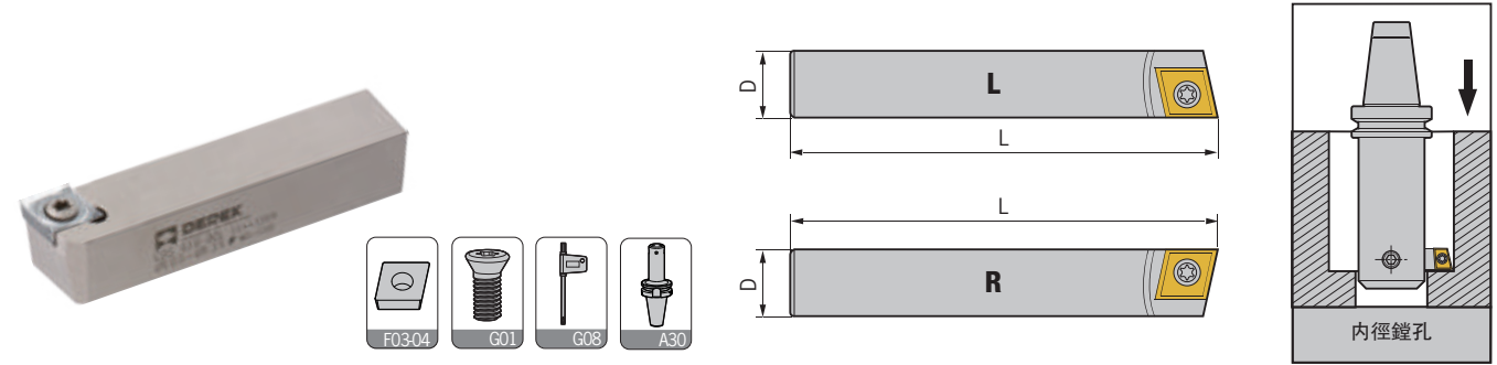
C90度刀杆適用於BSB刀柄 For BSB Boring Holder
